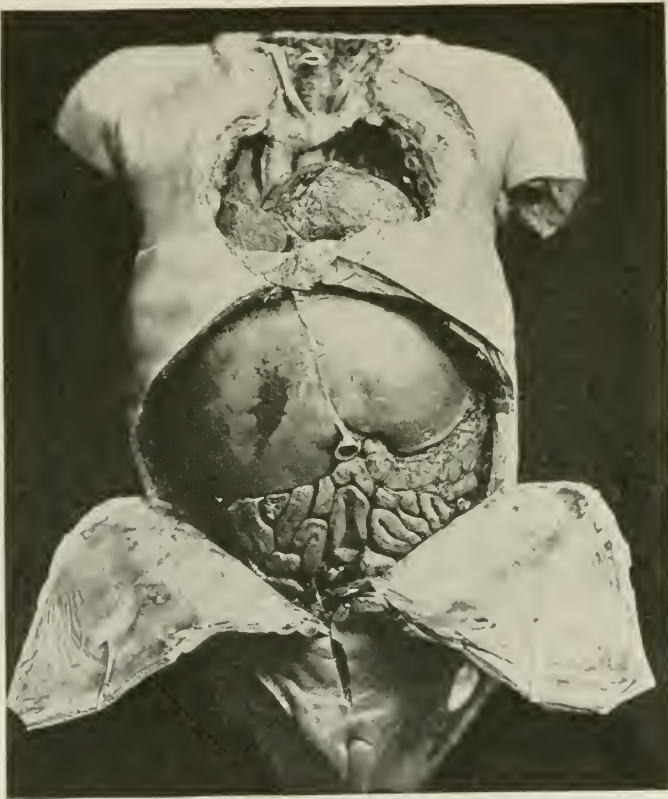
FIG. 115.—The infant's chest is circular in outline. The abdominal viscera are large. The proximity of the stomach and colon to the lower portion of the lungs imparts a tympanitic quality to the lower lobes, especially the left, and renders very light percussion essential. The heart lies almost horizontally, hence cardiac dullness extends relatively further to the left than is the case in adults. It also lies about one interspace higher in infants.
